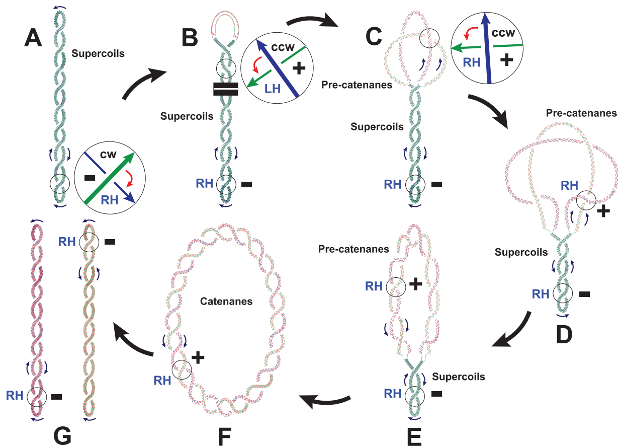
FIGURE 2 Cartoons illustrating the changes in topological sign and chirality that take place during the replication cycle. (A) Un-replicated negatively supercoiled form showing right-handed crossings with negative signs. (B) As replication starts, opening of the DNA double-helix generates positive supercoiling immediately ahead of the replication forks (upper part of the un-replicated region). The combined action of DNA gyrase, Topoisomerase IV and swivelling of the forks eliminate this positive torsional tension and keep the un-replicated region negatively supercoiled (lower part of the un-replicated region). (C) Swivelling of the forks diffuses some of the positive supercoiling that transiently accumulates immediately ahead of the forks from the un-replicated to the replicated region at the expense of generating right-handed positive crossings between the newly made sister duplexes. (D) As the replicating forks keep advancing the un-replicated negatively supercoiled region becomes smaller, and the size of the replicated region increases. At mid-replication both regions have approximately the same size, manifesting similar number of crossings. (E) At late replication stages, most of the molecule has been replicated, possessing numerous pre-catenane crossings in the replicated region and few negative supercoils in the un-replicated one. (F) Once replication finishes, the newly made sister duplexes remain heavily catenated. (G) Topoisomerase IV progressively eliminates catenation and allows the sister duplexes to segregate. The parental chains are represented in blue and green, while newly synthesized chains are depicted in red
